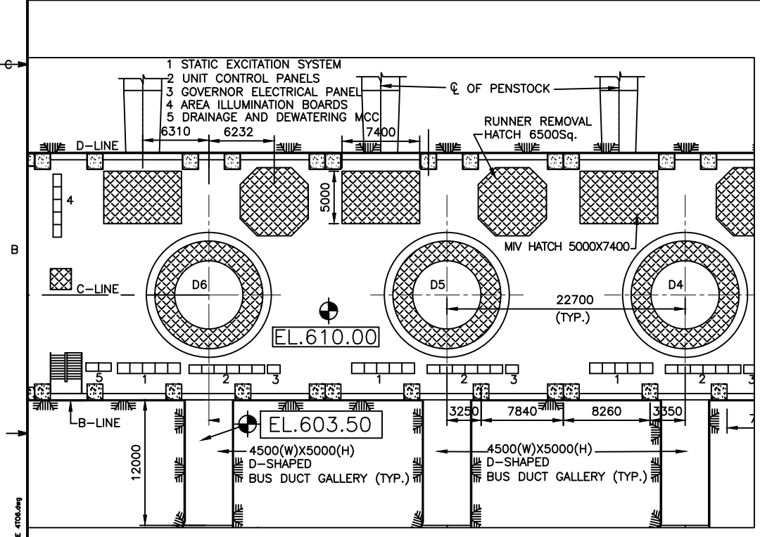
DETAIL-A
