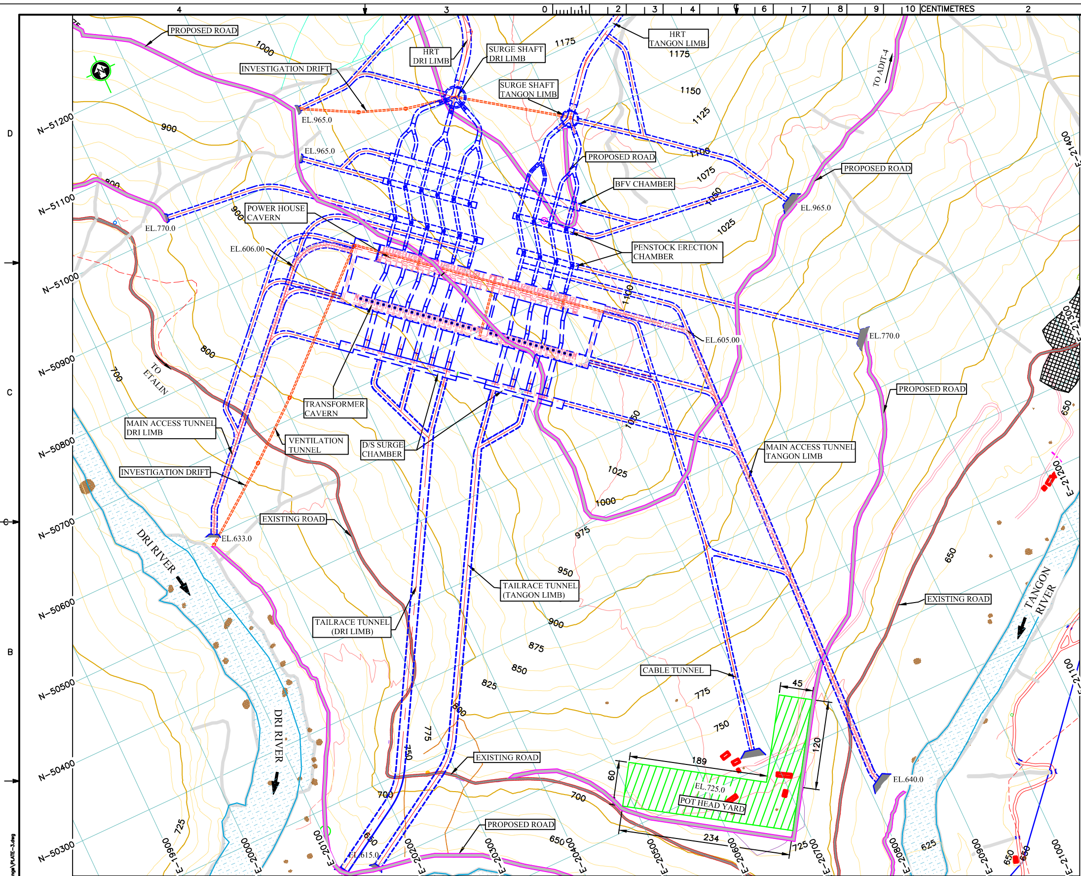
LAYOUT PLAN (SCALE 1:5000)
